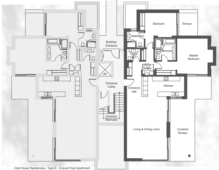
Club House Residences - Type B - Ground Floor Apartment
